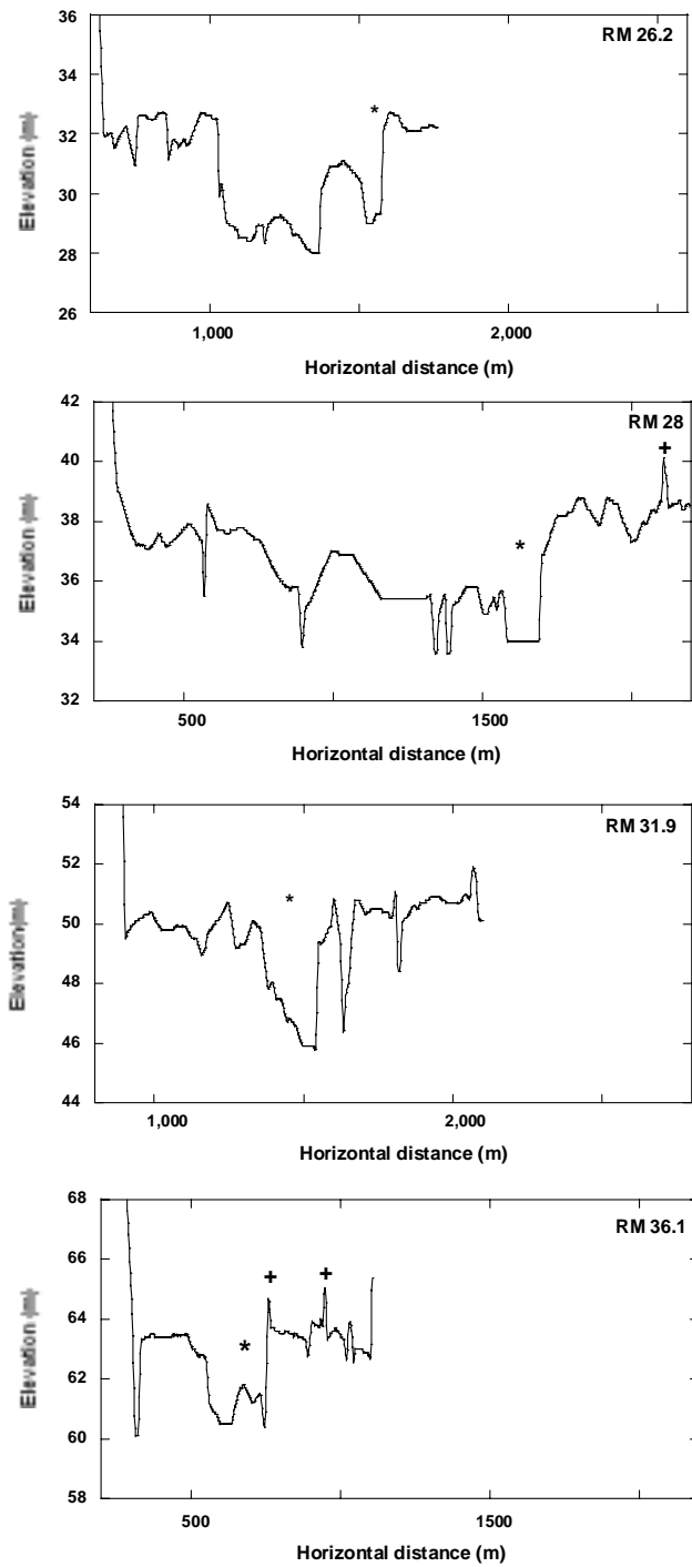
Figure 5B. Representative valley cross sections in the upper Nooksack River mainstem (RM24—RM37). Cross sections were created by sampling 2.5-m-cell size DEM created from 1993 photogrammetric data. “*” = Nooksack River; “+” = road. Vertical exaggeration = 100x.
