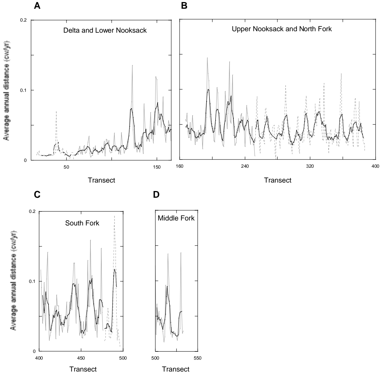
Figure 10. Average annual distance of lateral movement, for the period of aerial photo record (1933-2002), divided by the width of the active channel in 1998; distance is expressed as channel widths per year. Darker line represents a 1-km moving average of the 0.2-km spaced transect data. (A) Delta (dashed line) and lower Nooksack (solid line), (B) Upper Nooksack (solid line) and North Fork (dashed line), (C) South Fork (solid line) and upper South Fork (dashed line), and (D) Middle Fork. Transect numbers refer to Figure 1. Scale of vertical and horizontal axes is the same in each panel.
